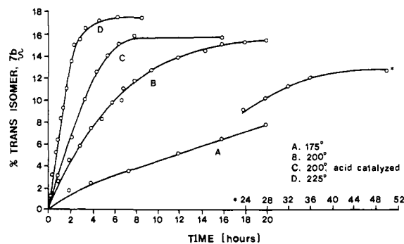
Figure 4. Equilibration of r -2-phenyl- c -5- tert -butyl-1,3,2-dithiaphosphorinane ( 7a ).
