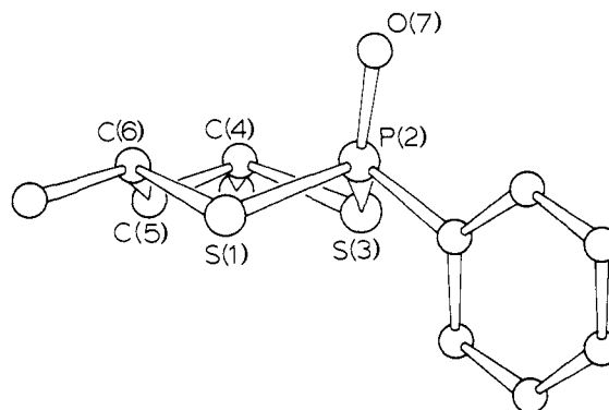
Figure 9. Structure and solid-state conformation of 22 .
