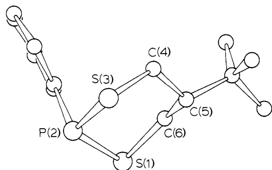
Figure 1. Structure and solid-state conformation of 7a .
