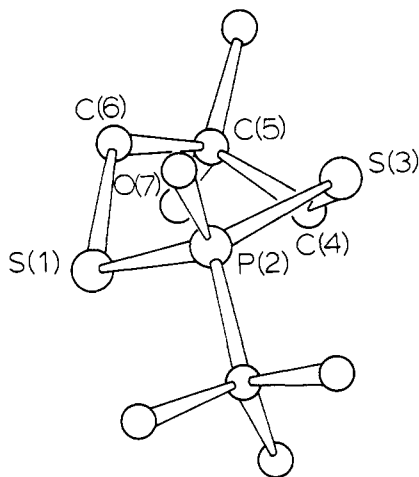
Figure 12. Structure and solid-state conformation of 28 .
