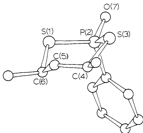
Figure 10. Structure and solid-state conformation of 23 .
