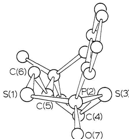
Figure 6. Structure and solid-state conformation of 6 .
