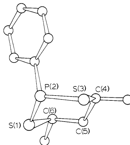
Figure 2. Structure and solid-state conformation of 11b .
