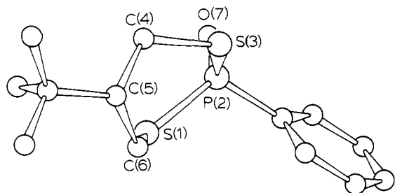
Figure 5. Structure and solid-state conformation of 5 .
