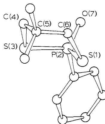
Figure 11. Structure and solid-state conformation of 24 .
