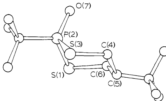
Figure 7. Structure and solid-state conformation of 19 .
