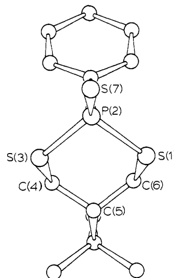
Figure 8. Structure and solid-state conformation of 20a .
