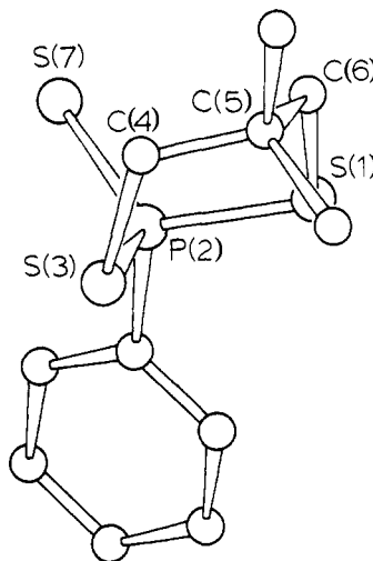
Figure 13. Structure and solid-state conformation of 31 .
